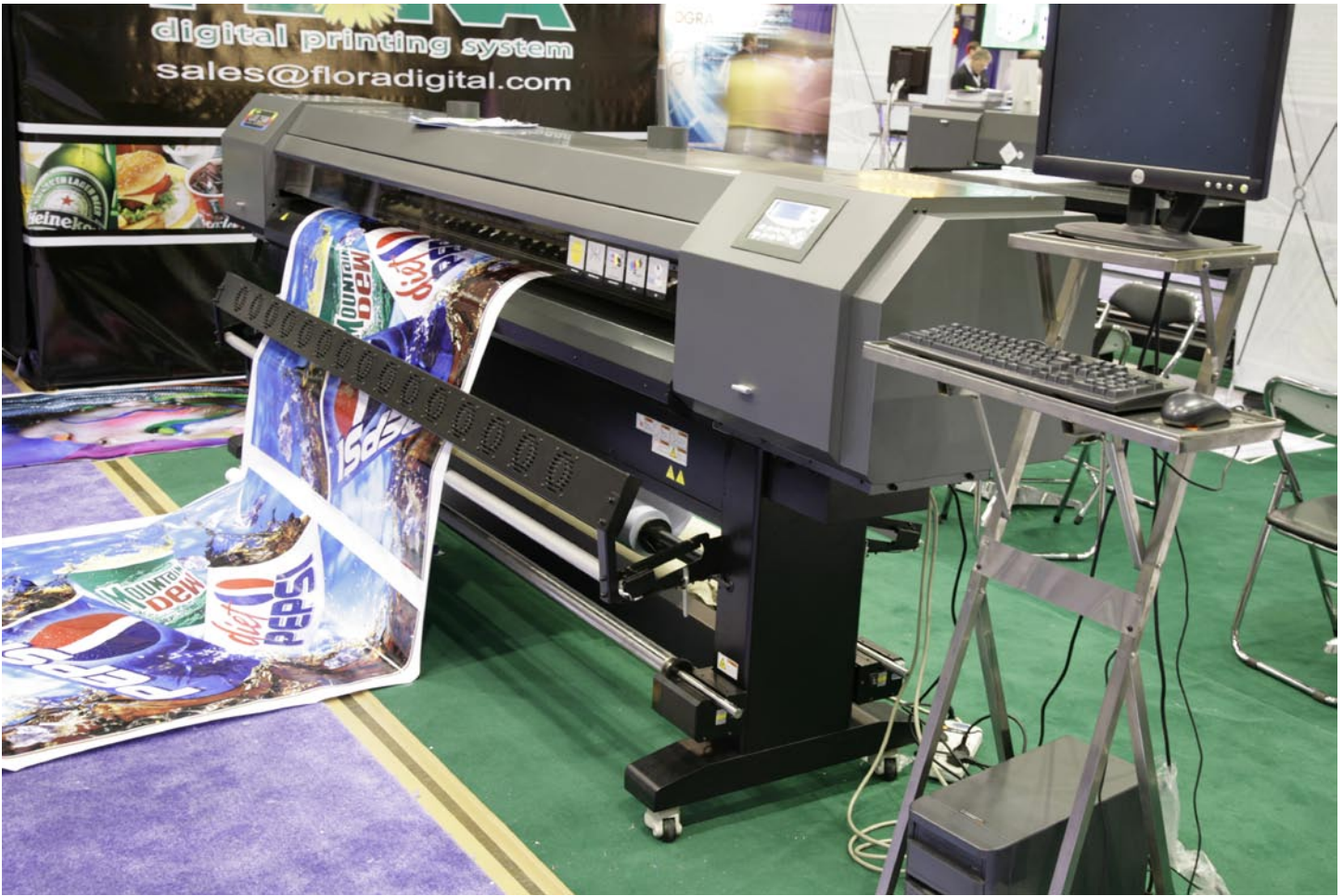
Two of the solvent printers from the Flora series (above and below left: 2500, below right: 3200)
